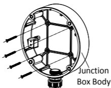
Figure 2-15 Secure the Junction Box's Body on Ceiling
