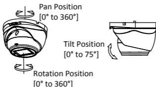
Figure 2-12 3-axis Adjustment
