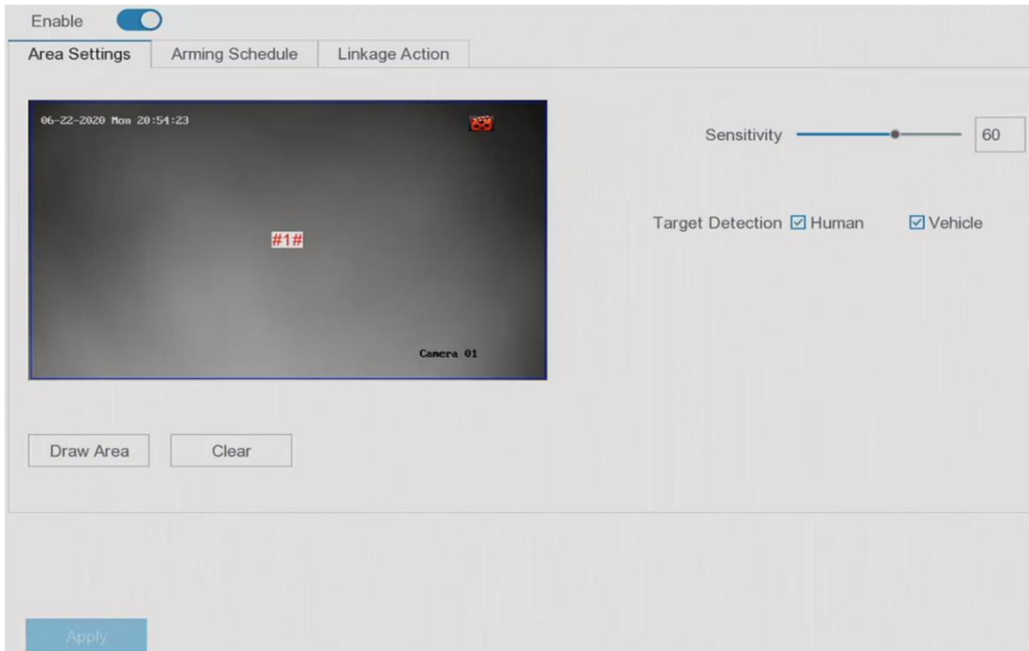
Figure 5-11 Motion Detection
