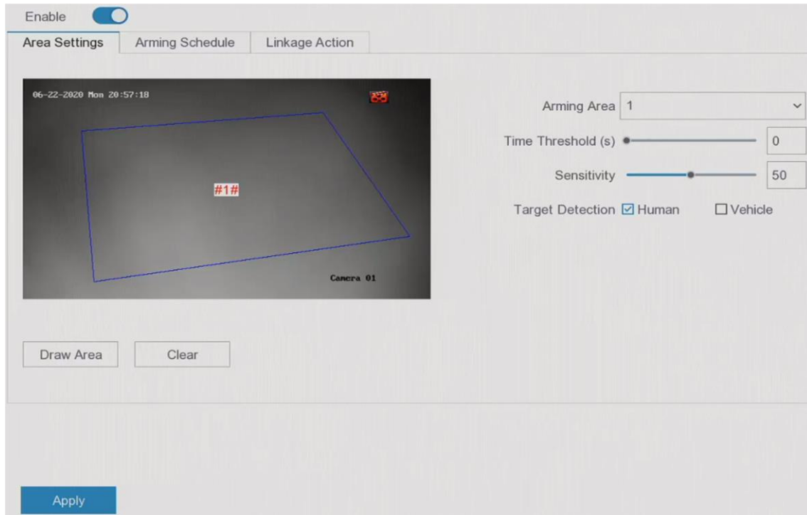
Figure 5-13 Intrusion Detection
